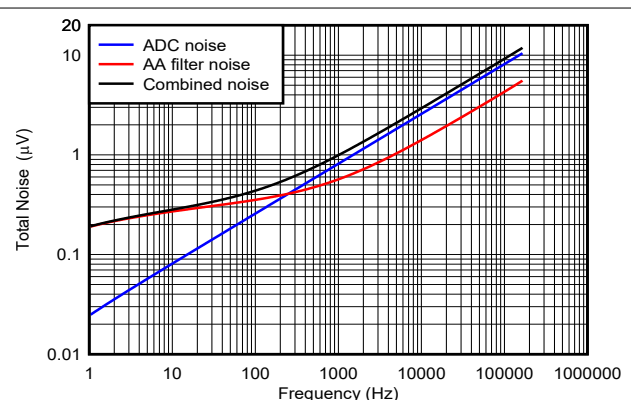
Figure 9-5. Total Noise
