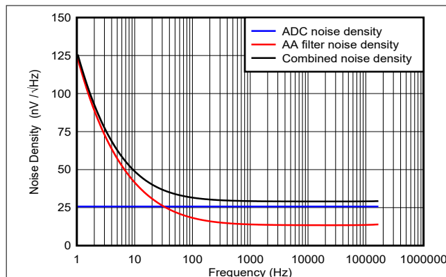
Figure 9-4. Noise Density
