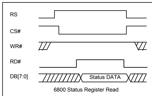
Figure 6-27 : 6800 Read Status Register
