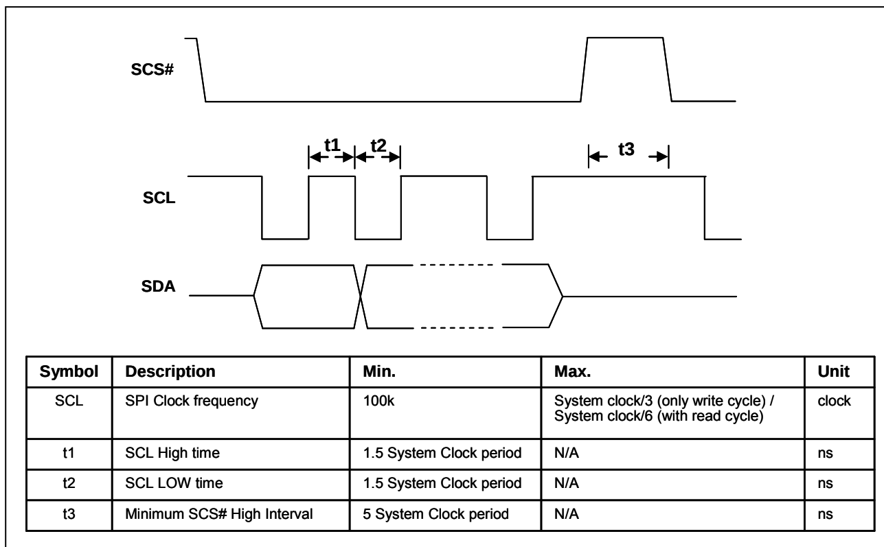
Figure 6-12 : 3-Wire SPI Timing
