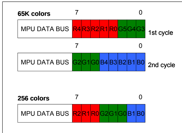
Figure 6-34 : Color illustrations for 8-Bit Data Bus MCU
