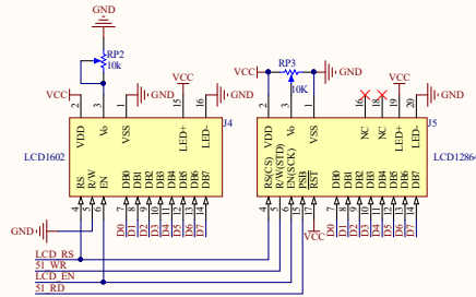
1602液晶&12864
